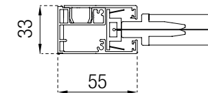
Guide Zip Z55 Z55 zip guides
