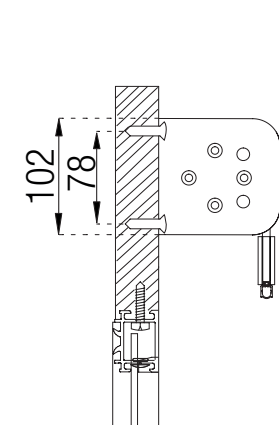
Livorno 102 attacco frontale Livorno 102 wall mounting
